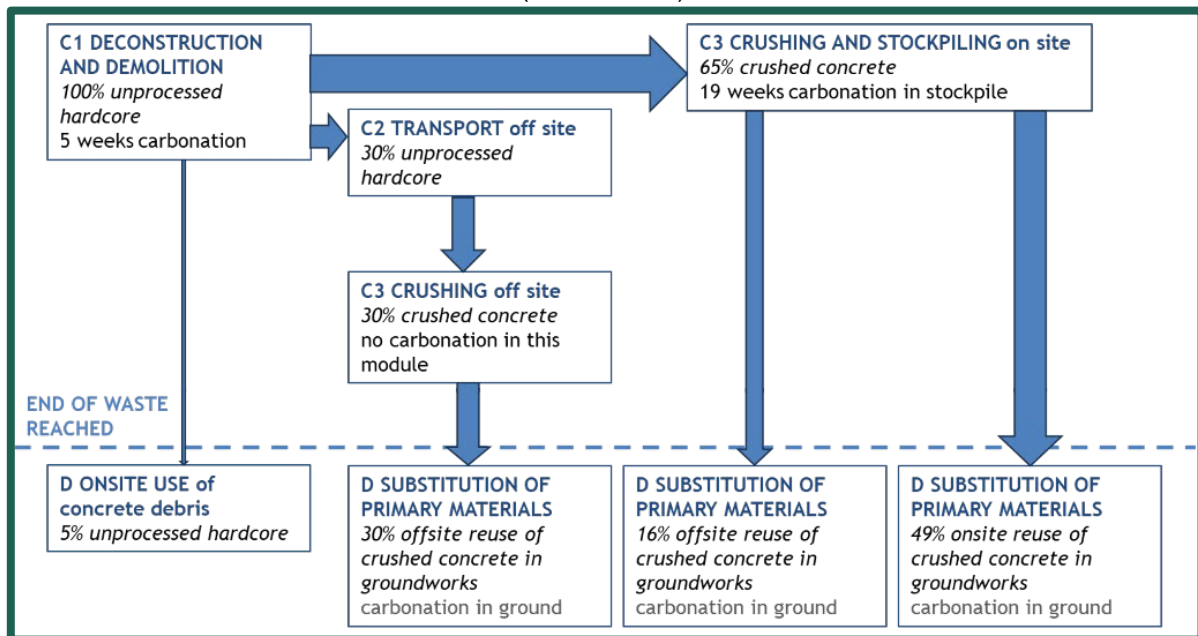
Figure 3. Typical flows of end-of-life concrete during modules C and D in reference to carbonation (NFDC, 2023).
